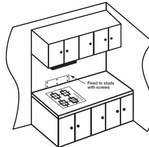
Figure : Installation of mineral board onto stud wall with self-tapping screws into the studs
